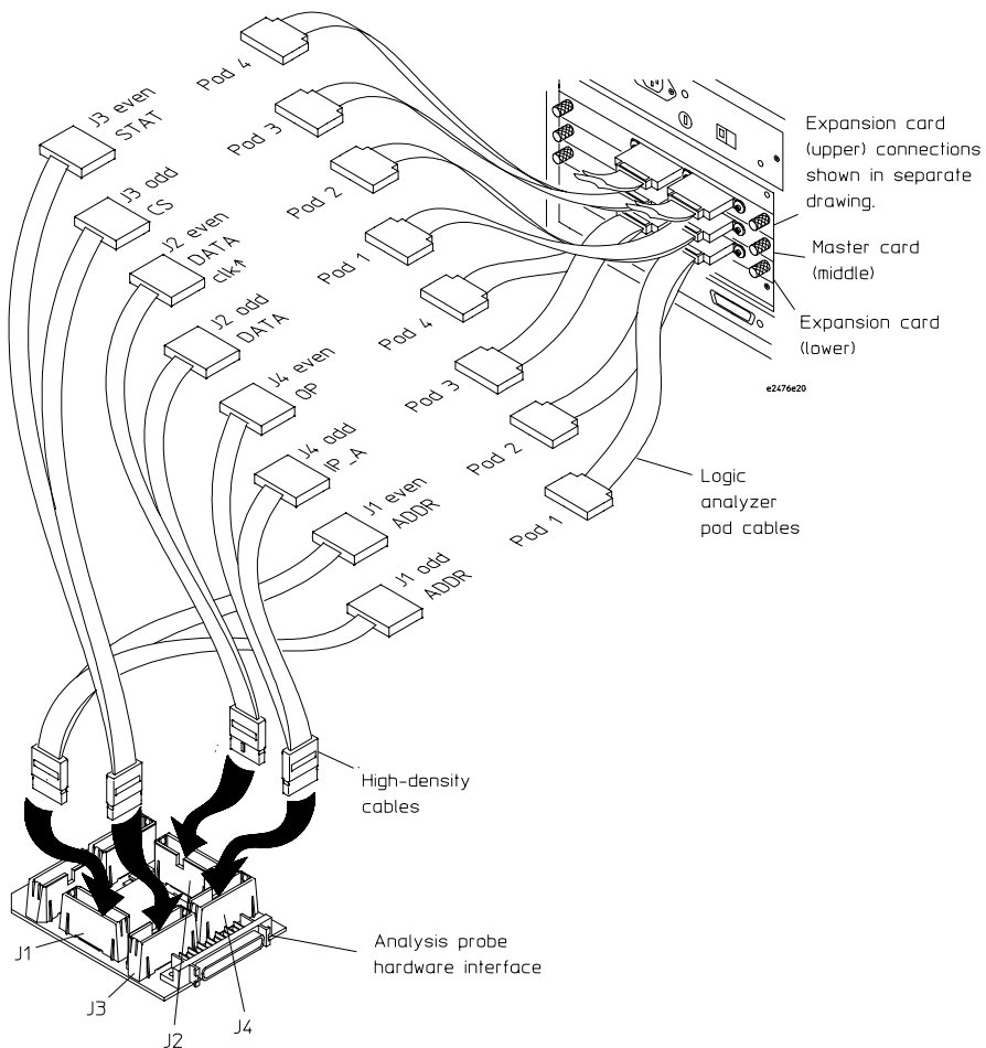
HP 16554/55/56/57 analyzer three-card analyzer connections, part 1
